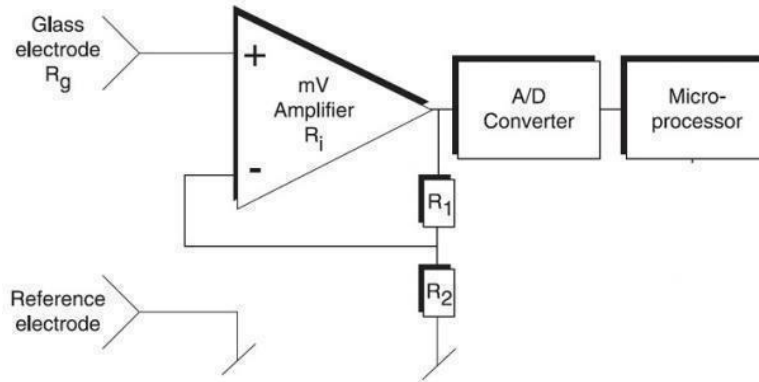
Figure 4: Inner Block of pH
