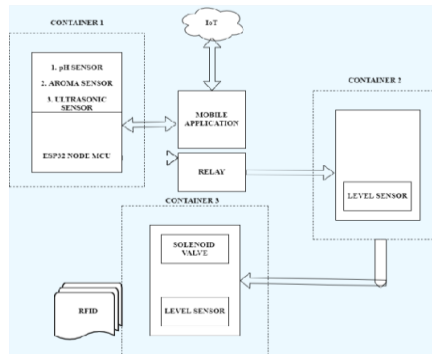
Figure 1: Block diagram
