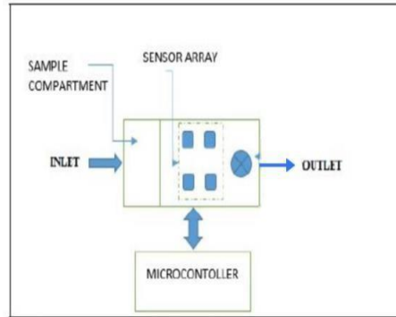
Figure 6: Block Diagram of Aroma Sensor
