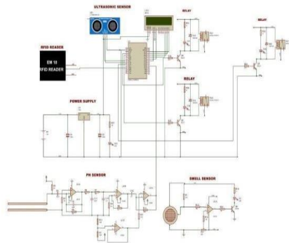
Figure 2: Circuit Diagram
